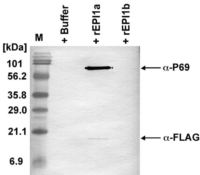
Figure 5 Coimmunoprecipitation of the recombinant Kazal domains and P69 subtilisins using FLAG antisera. Eluates from coimmunoprecipitation of rEPI1a, rEPI1b or buffer with proteins in BTH-treated tomato intercellular fluids were run on SDS-PAGE gel followed by sequential immunoblotting with P69 ( \alpha -P69) and FLAG ( \alpha -FLAG) antisera at a dilution of 1:3000.
